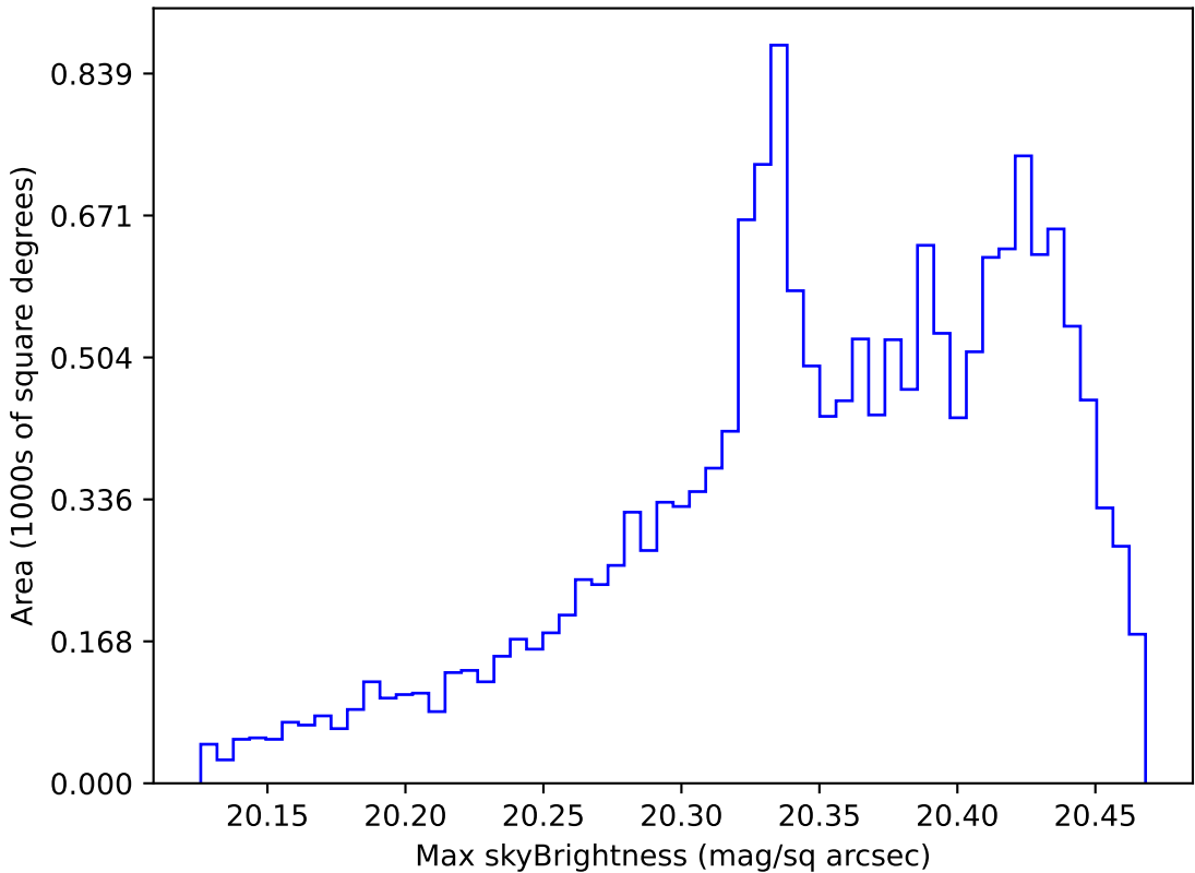
ddf_loaded_half_fl1_v3.4_10yrs WFD i band: Max skyBrightness
