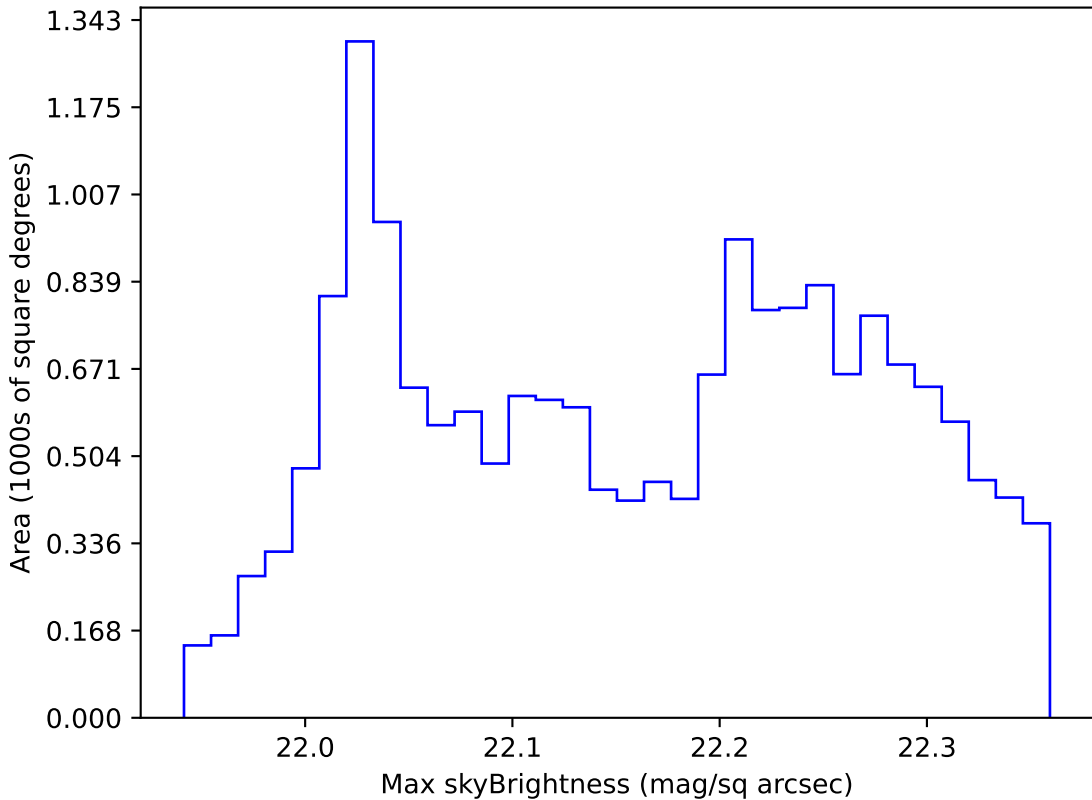
ddf_loaded_half_fl1_v3.4_10yrs WFD g band: Max skyBrightness
