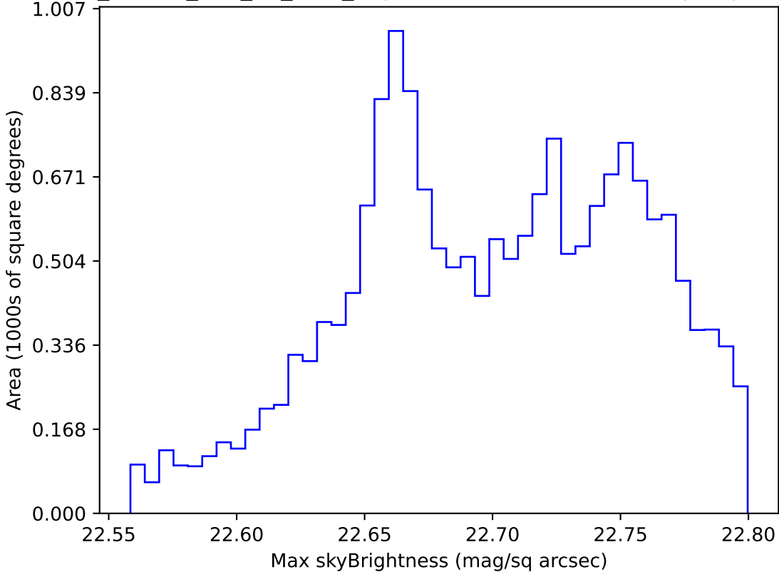
ddf_loaded_half_fl1_v3.4_10yrs WFD all bands: Max skyBrightness
