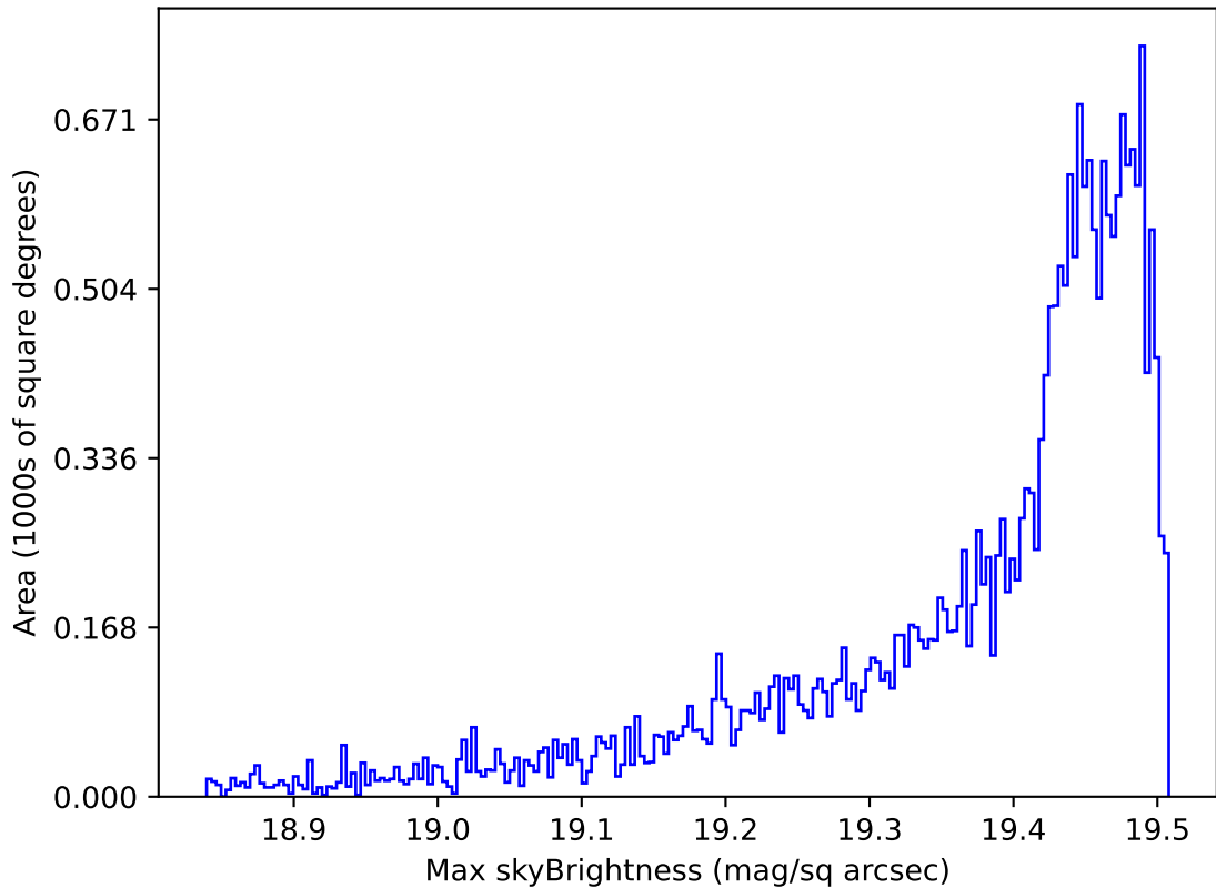
ddf_loaded_half_fl1_v3.4_10yrs All sky z band: Max skyBrightness
