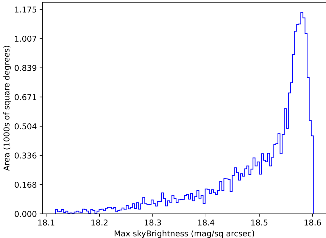
ddf_loaded_half_fl1_v3.4_10yrs All sky y band: Max skyBrightness
