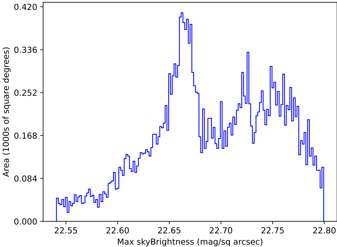
ddf_loaded_half_fl1_v3.4_10yrs All sky u band: Max skyBrightness
