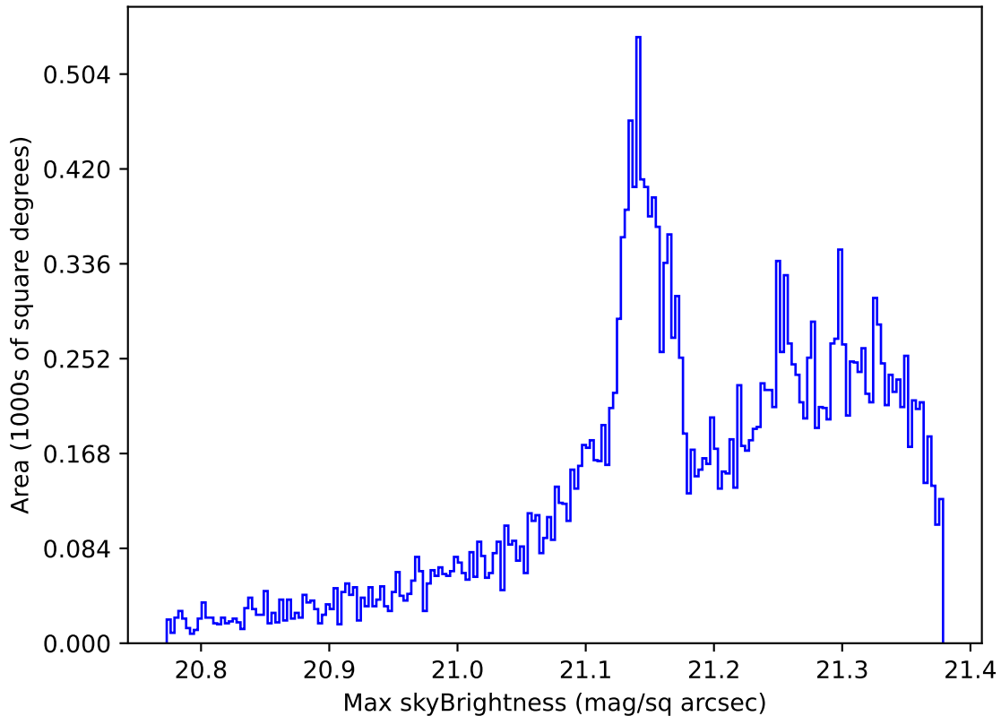
ddf_loaded_half_fl1_v3.4_10yrs All sky r band: Max skyBrightness
