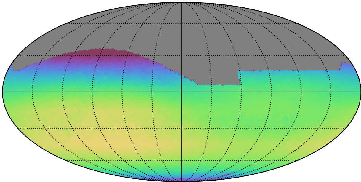
ddf_loaded_half_fl1_v3.4_10yrs All sky i band: Max skyBrightness
