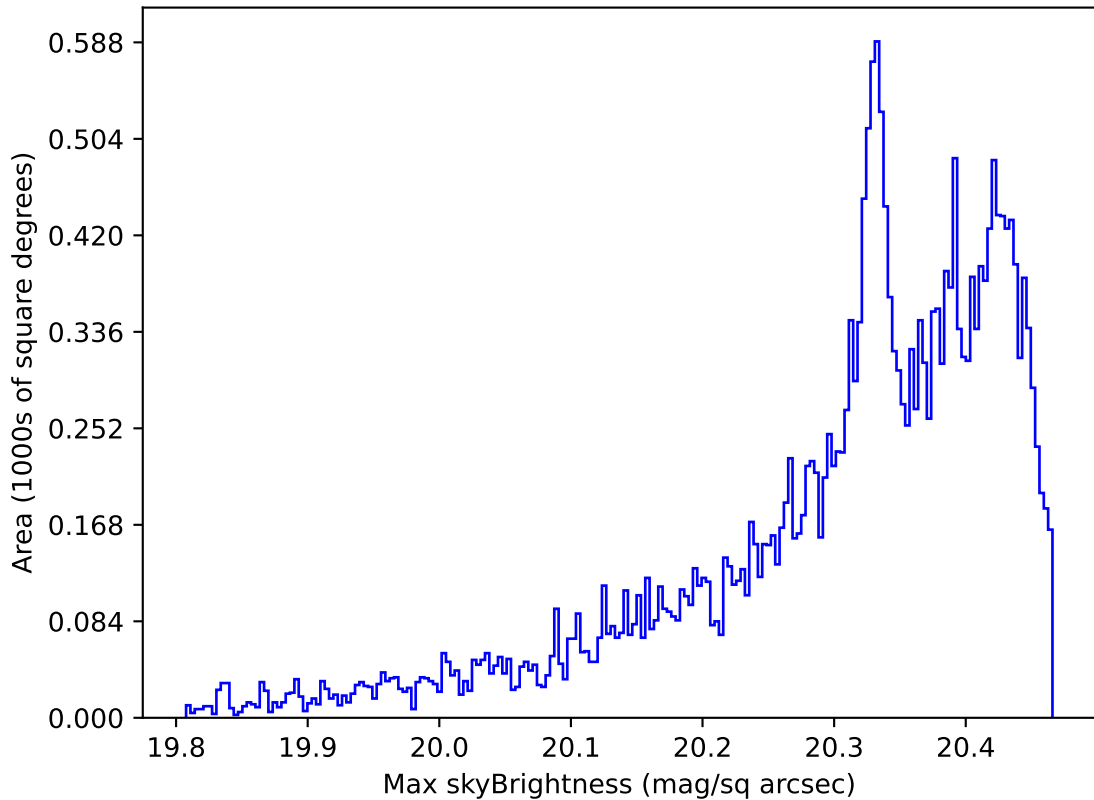
ddf_loaded_half_fl1_v3.4_10yrs All sky i band: Max skyBrightness
