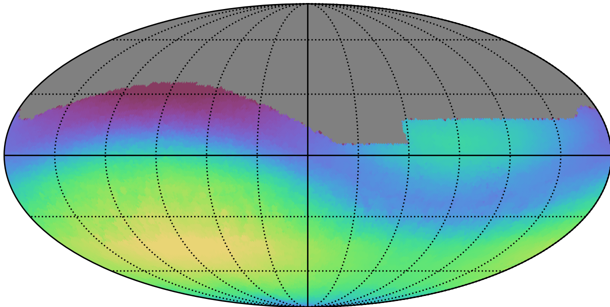
ddf_loaded_half_fl1_v3.4_10yrs All sky g band: Max skyBrightness
