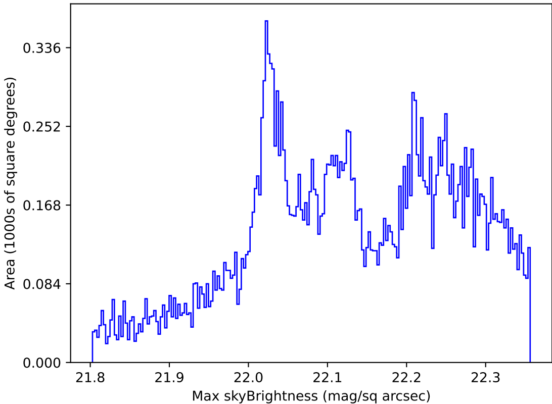
ddf_loaded_half_fl1_v3.4_10yrs All sky g band: Max skyBrightness
