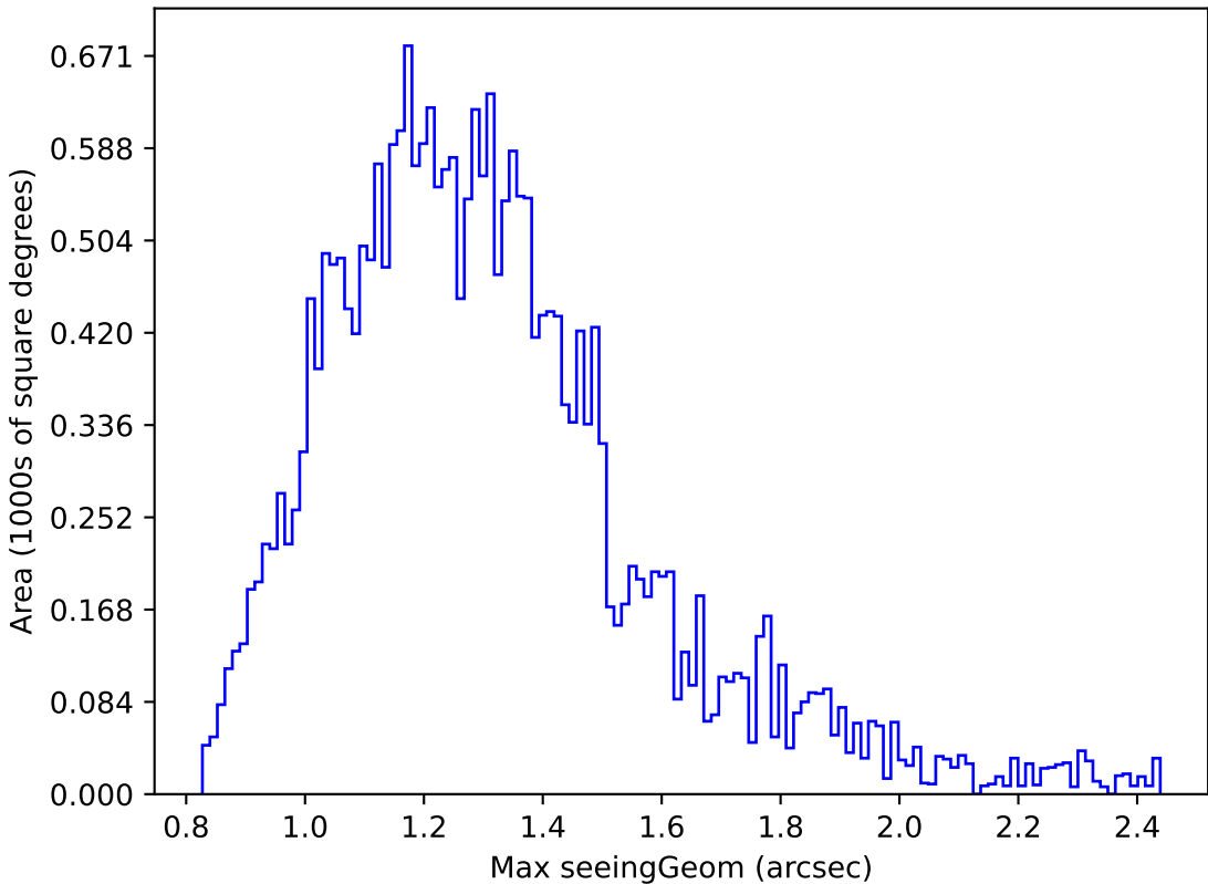
ddf_loaded_half_fl1_v3.4_10yrs Yr 1 z band: Max seeingGeom
