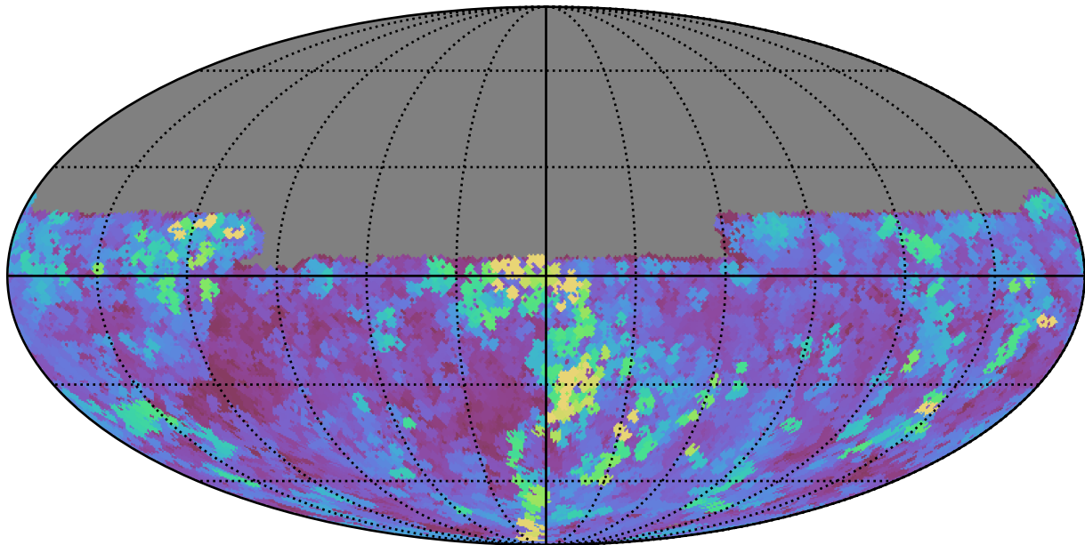
ddf_loaded_half_fl1_v3.4_10yrs Yr 1 y band: Max seeingGeom
