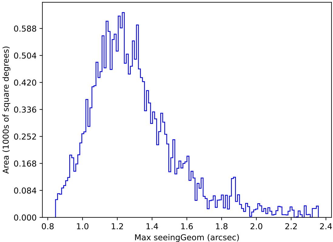
ddf_loaded_half_fl1_v3.4_10yrs Yr 1 y band: Max seeingGeom
