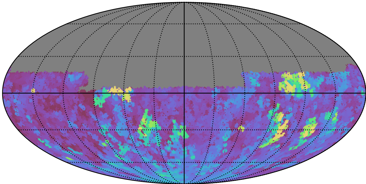
ddf_loaded_half_fl1_v3.4_10yrs Yr 1 u band: Max seeingGeom
