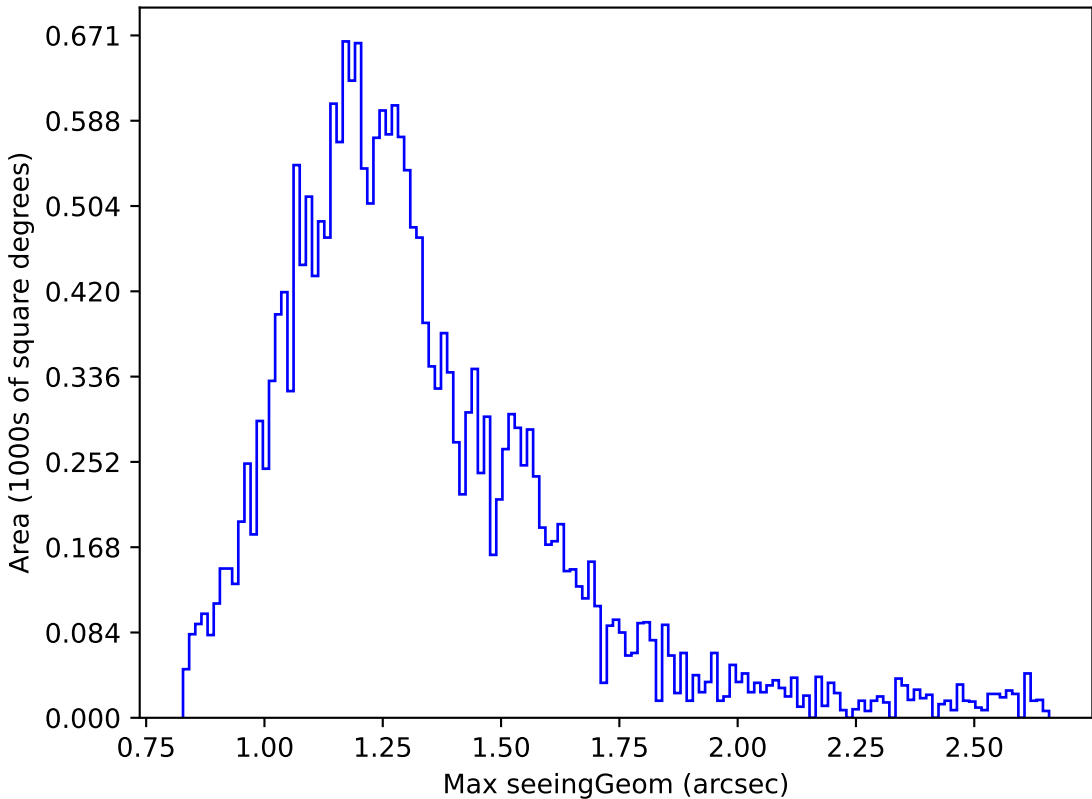
ddf_loaded_half_fl1_v3.4_10yrs Yr 1 u band: Max seeingGeom
