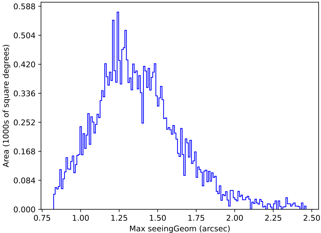
ddf_loaded_half_fl1_v3.4_10yrs Yr 1 r band: Max seeingGeom
