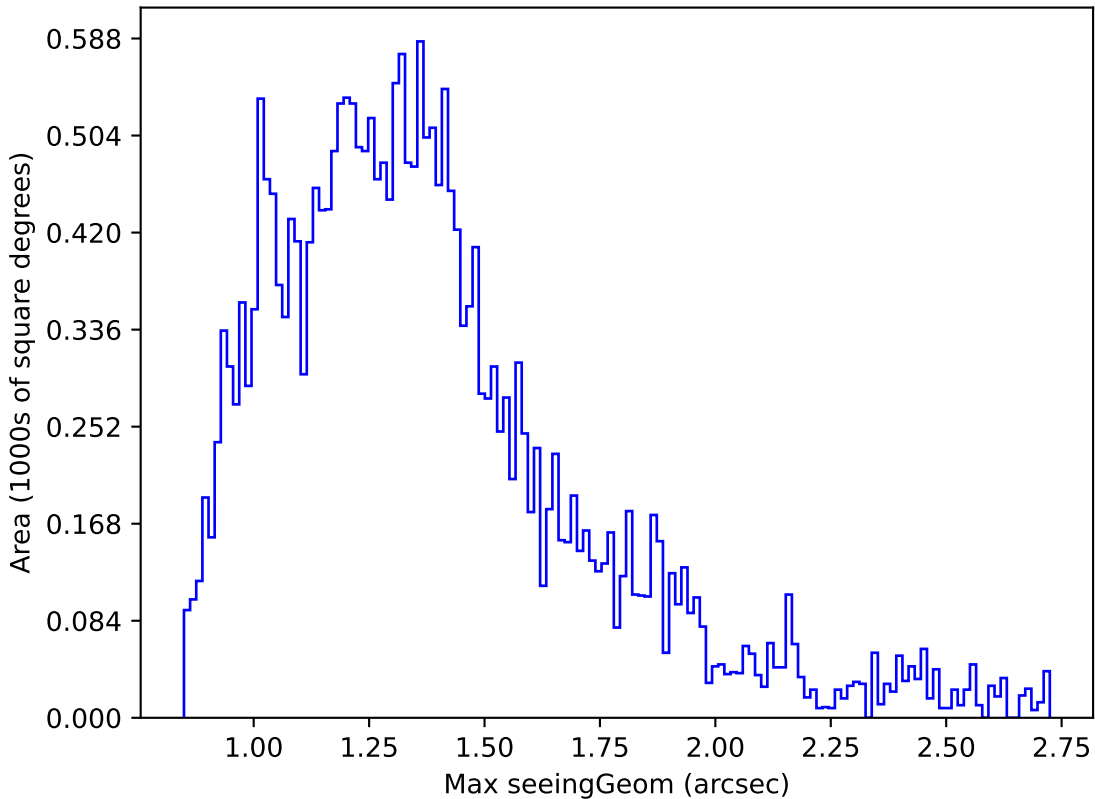
ddf_loaded_half_fl1_v3.4_10yrs Yr 1 i band: Max seeingGeom
