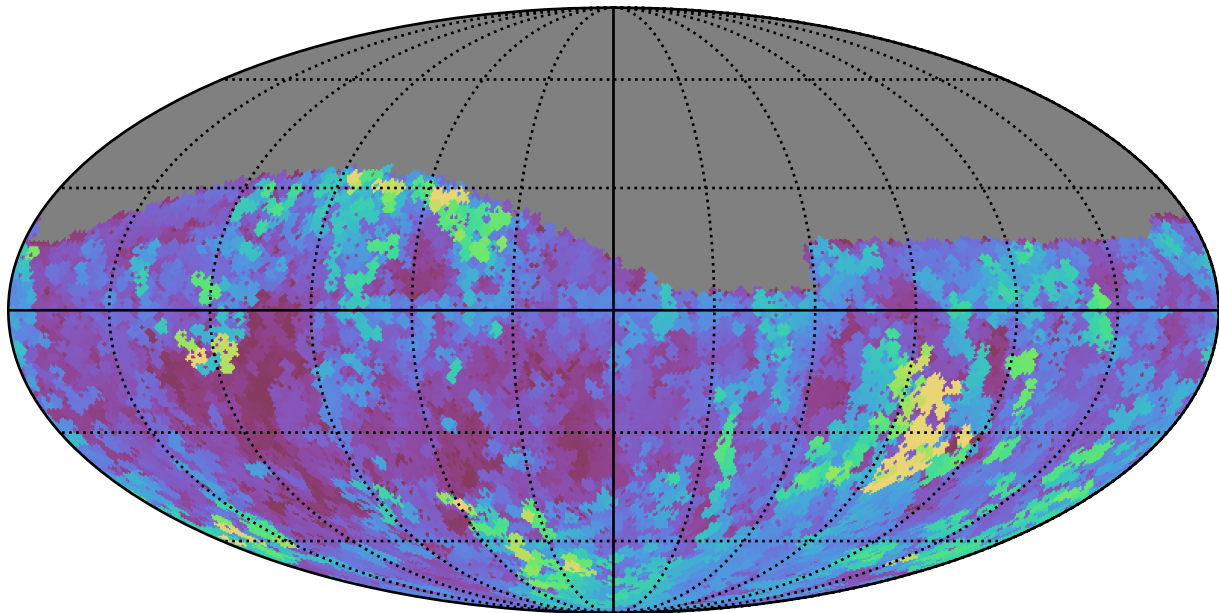
ddf_loaded_half_fl1_v3.4_10yrs Yr 1 g band: Max seeingGeom
