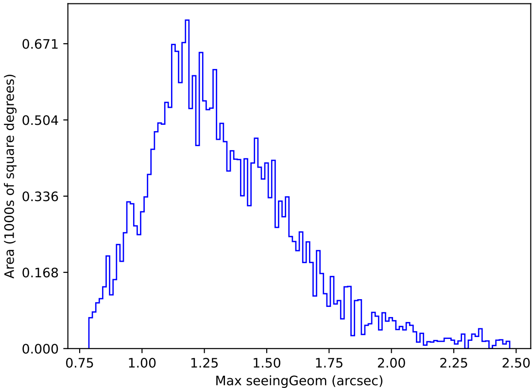
ddf_loaded_half_fl1_v3.4_10yrs Yr 1 g band: Max seeingGeom
