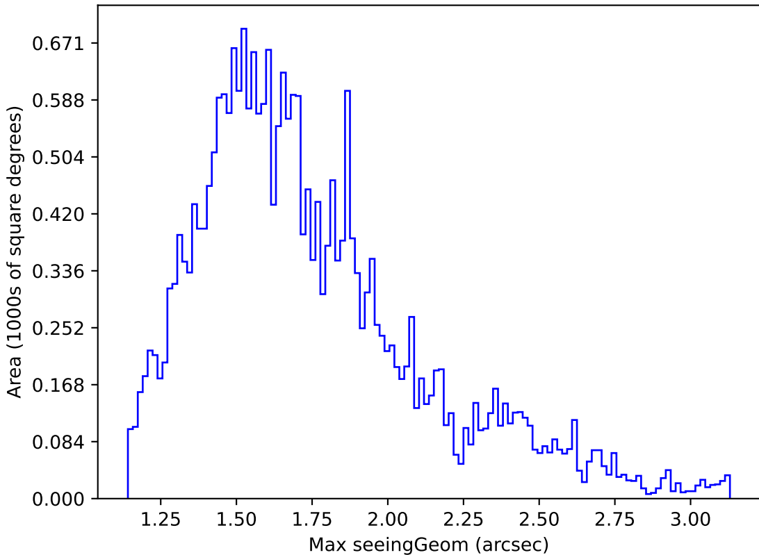
ddf_loaded_half_fl1_v3.4_10yrs Yr 1 all bands: Max seeingGeom
