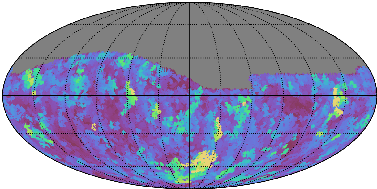
ddf_loaded_half_fl1_v3.4_10yrs Yr 1 z band: Max seeingEff
