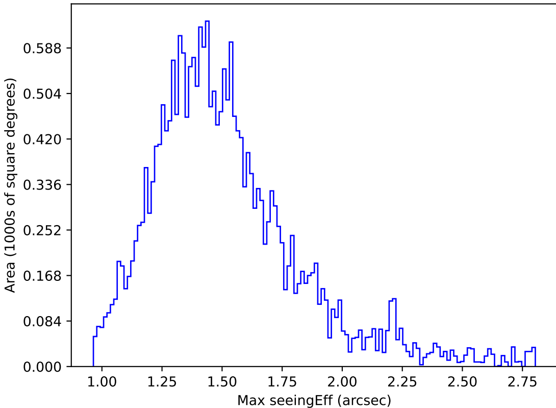
ddf_loaded_half_fl1_v3.4_10yrs Yr 1 y band: Max seeingEff
