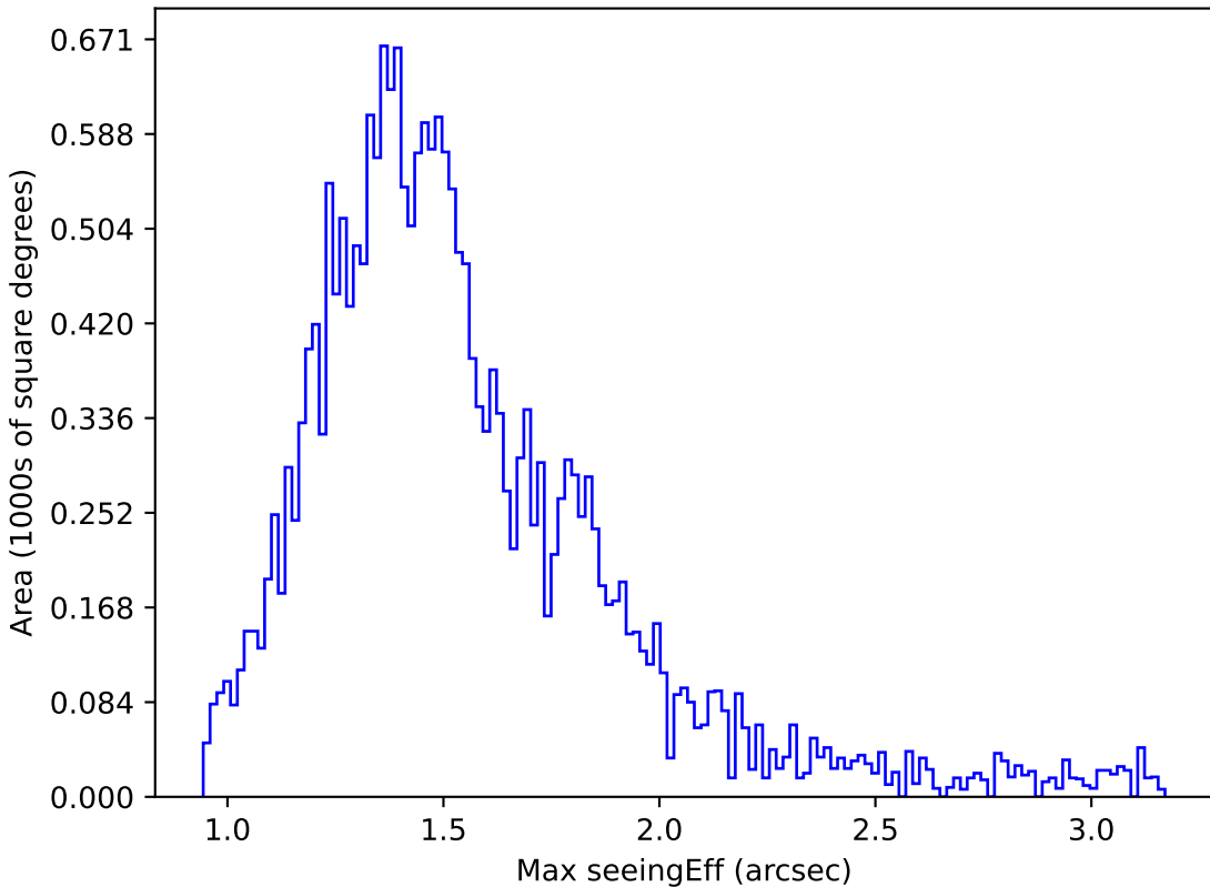
ddf_loaded_half_fl1_v3.4_10yrs Yr 1 u band: Max seeingEff
