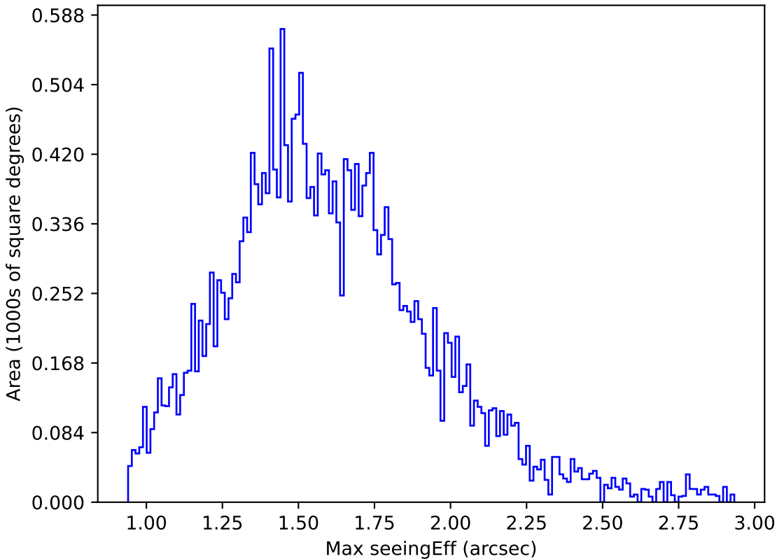
ddf_loaded_half_fl1_v3.4_10yrs Yr 1 r band: Max seeingEff
