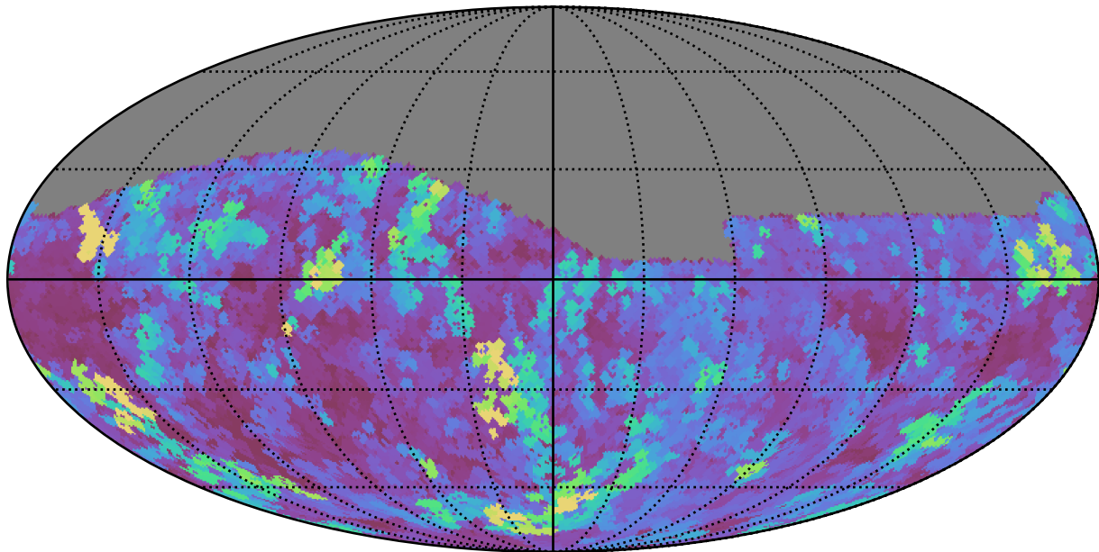
ddf_loaded_half_fl1_v3.4_10yrs Yr 1 i band: Max seeingEff
