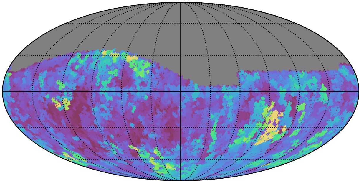
ddf_loaded_half_fl1_v3.4_10yrs Yr 1 g band: Max seeingEff
