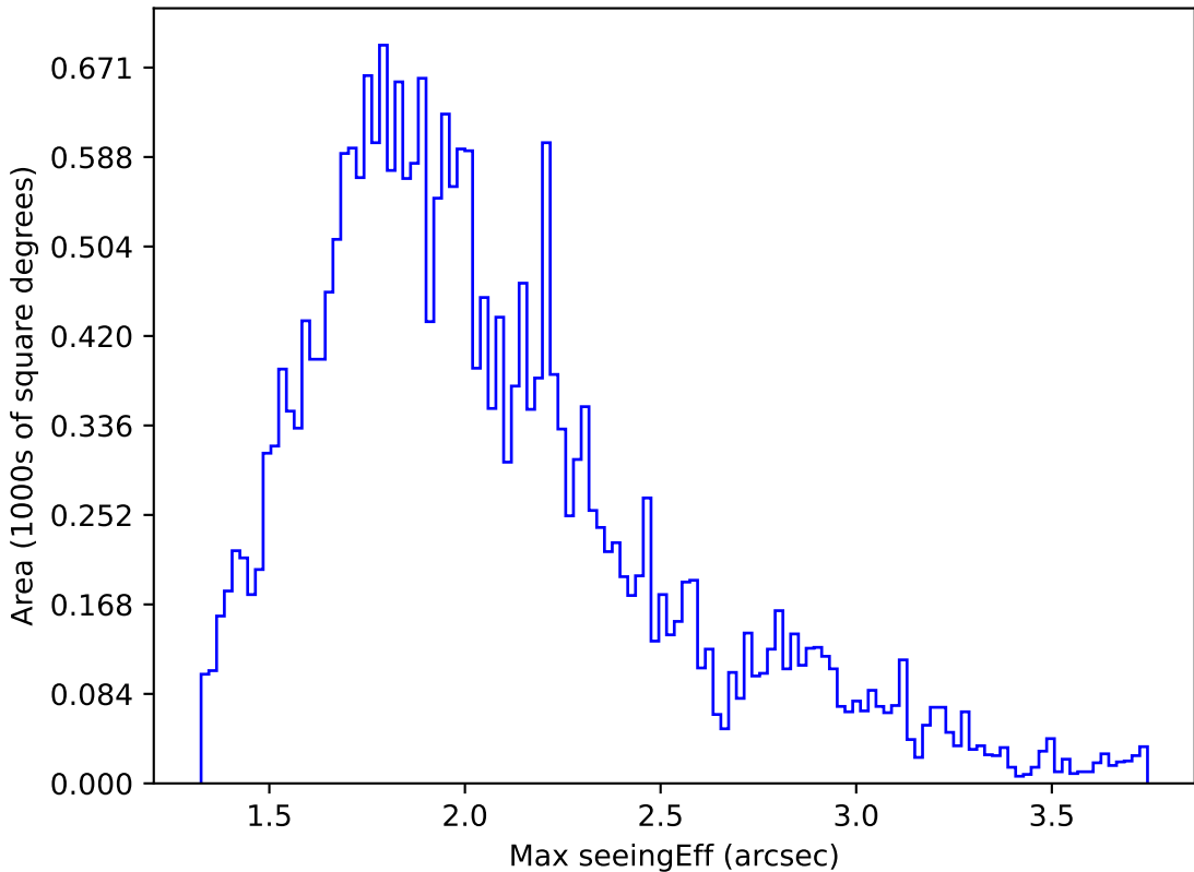
ddf_loaded_half_fl1_v3.4_10yrs Yr 1 all bands: Max seeingEff
