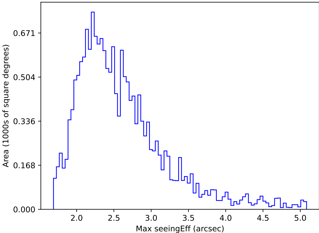
ddf_loaded_half_fl1_v3.4_10yrs WFD z band: Max seeingEff
