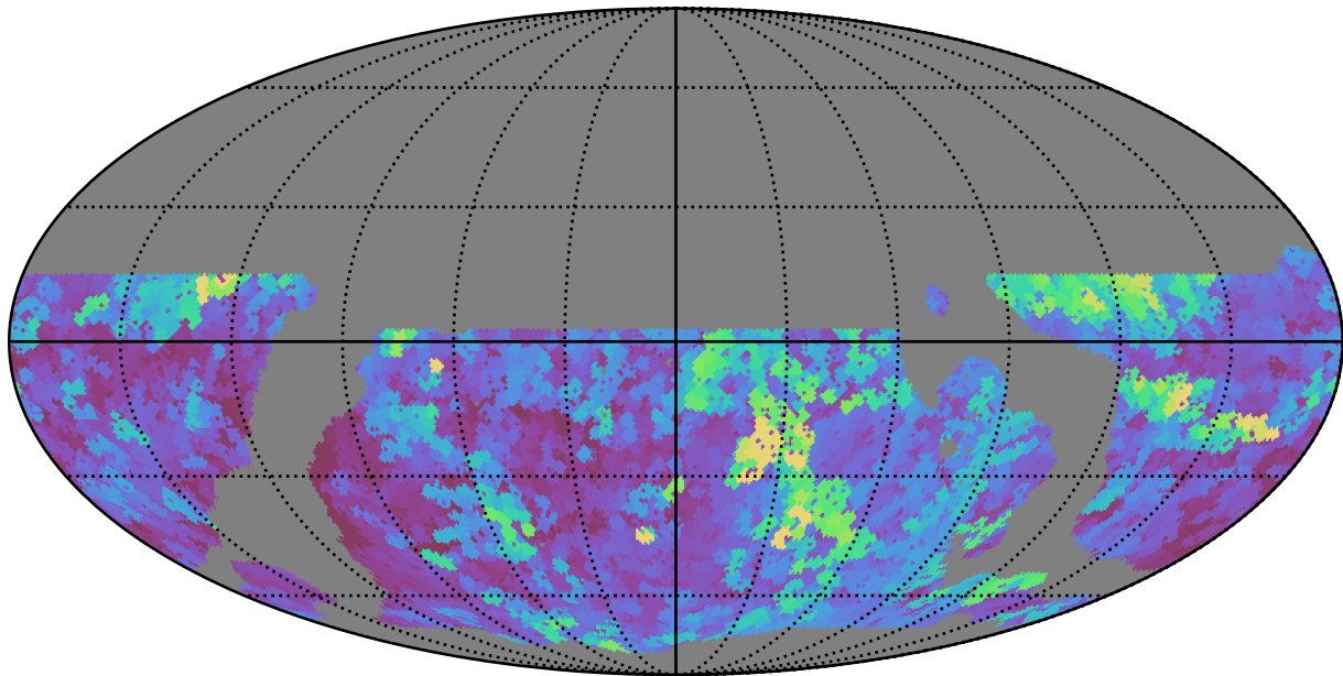
ddf_loaded_half_fl1_v3.4_10yrs WFD r band: Max seeingEff
