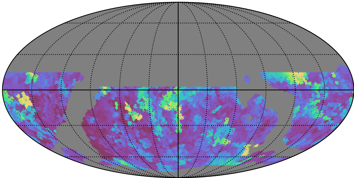
ddf_loaded_half_fl1_v3.4_10yrs WFD i band: Max seeingEff
