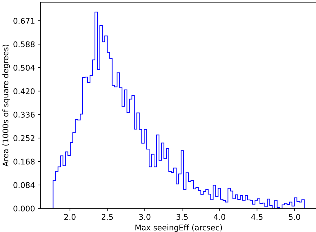
ddf_loaded_half_fl1_v3.4_10yrs WFD i band: Max seeingEff
