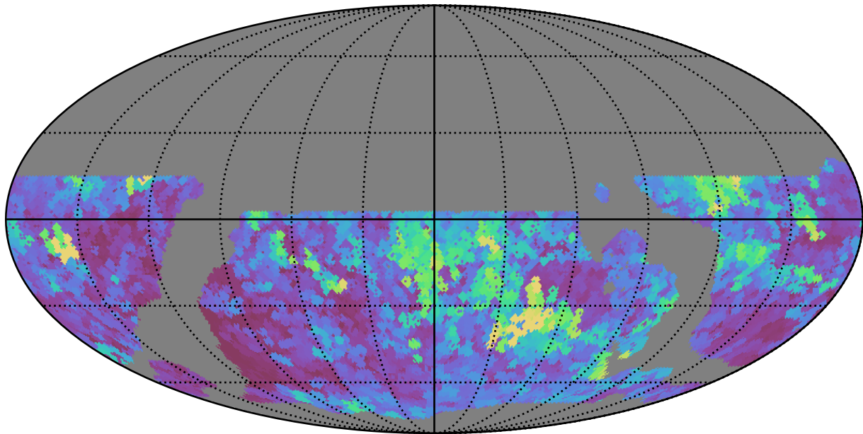
ddf_loaded_half_fl1_v3.4_10yrs WFD all bands: Max seeingEff
