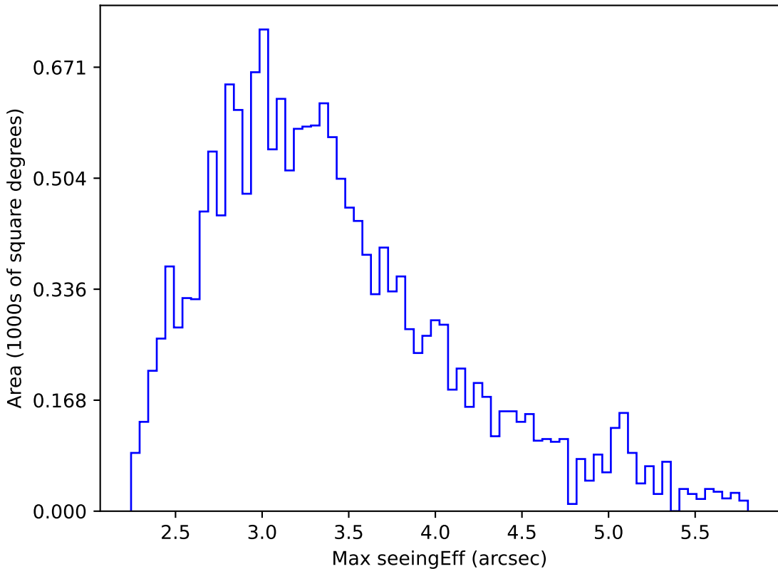
ddf_loaded_half_fl1_v3.4_10yrs WFD all bands: Max seeingEff
