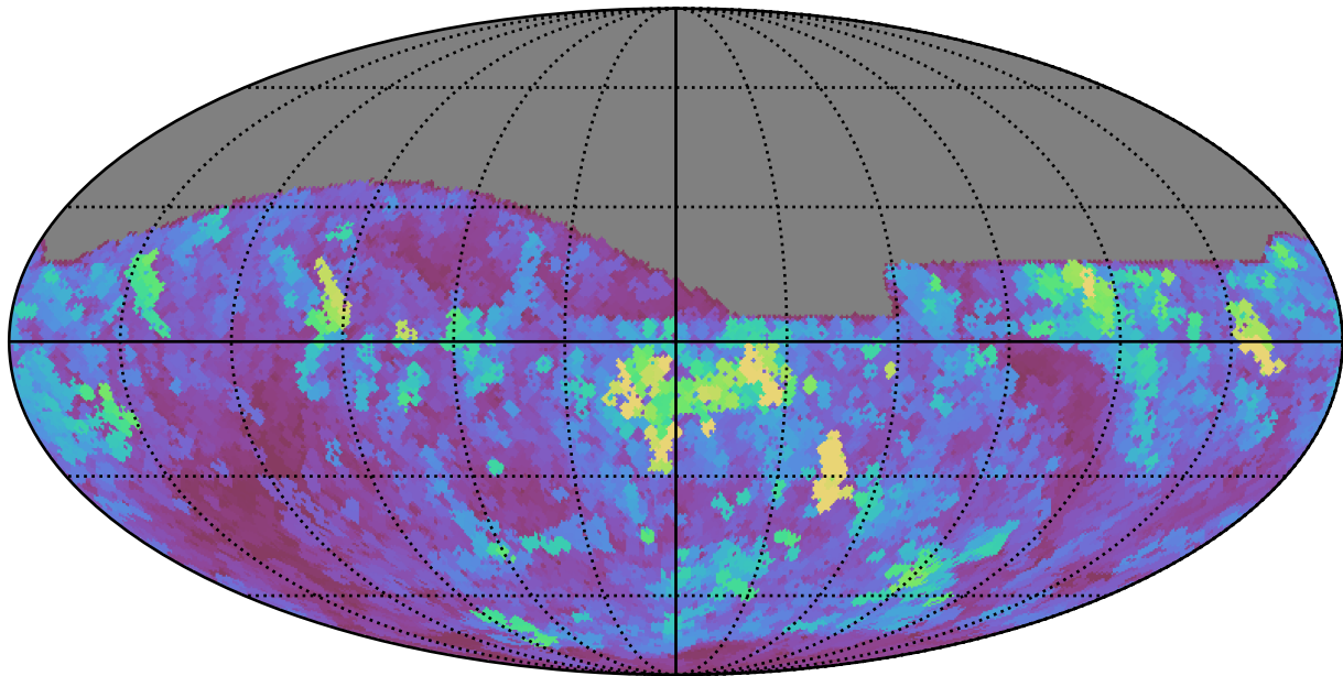
ddf_loaded_half_fl1_v3.4_10yrs All sky z band: Max seeingEff
