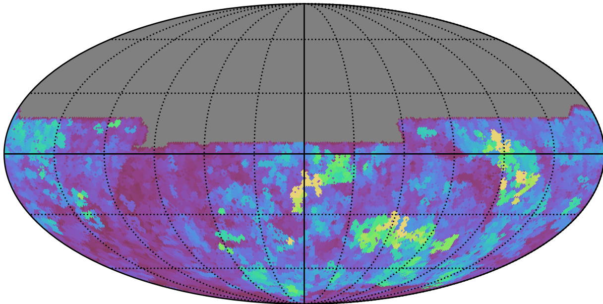
ddf_loaded_half_f11_v3.4_10yrs All sky y band: Max seeingEff
