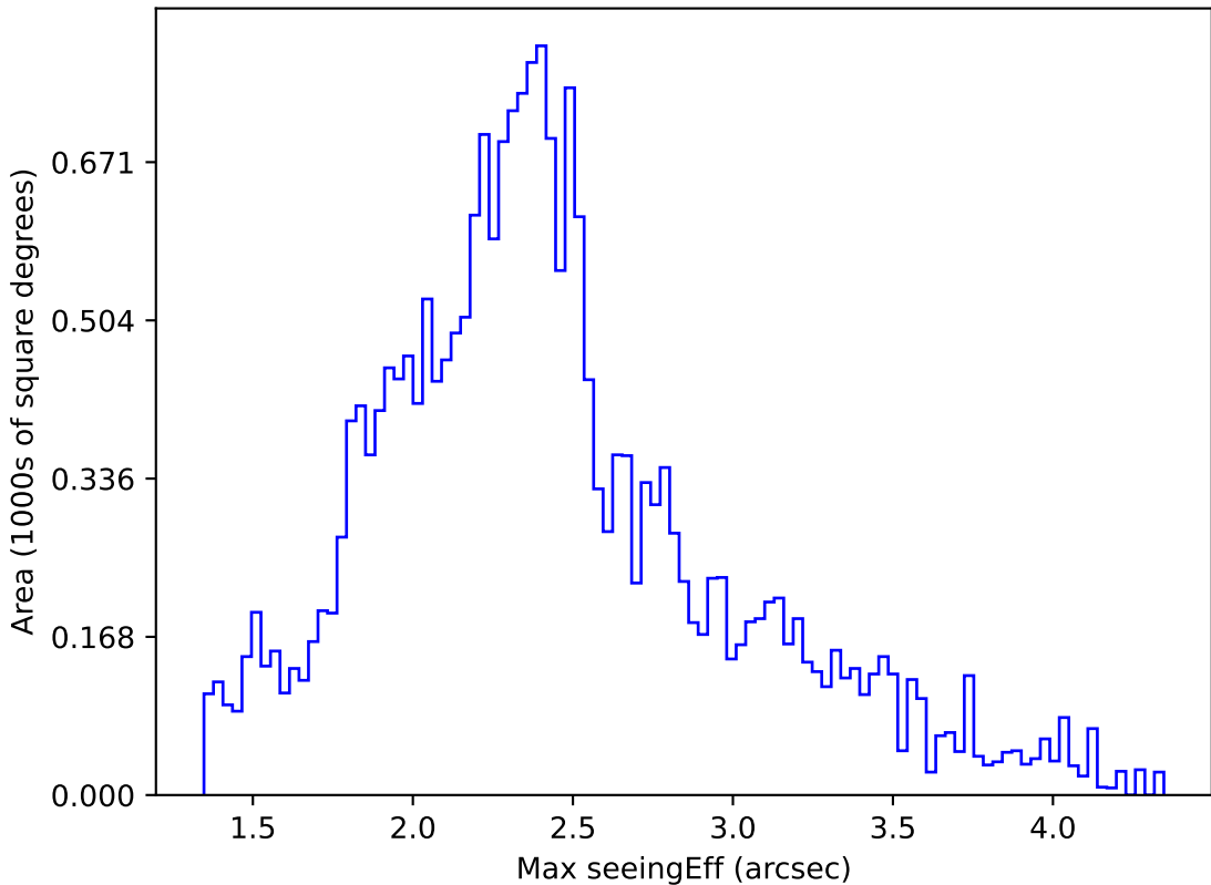
ddf_loaded_half_fl1_v3.4_10yrs All sky u band: Max seeingEff
