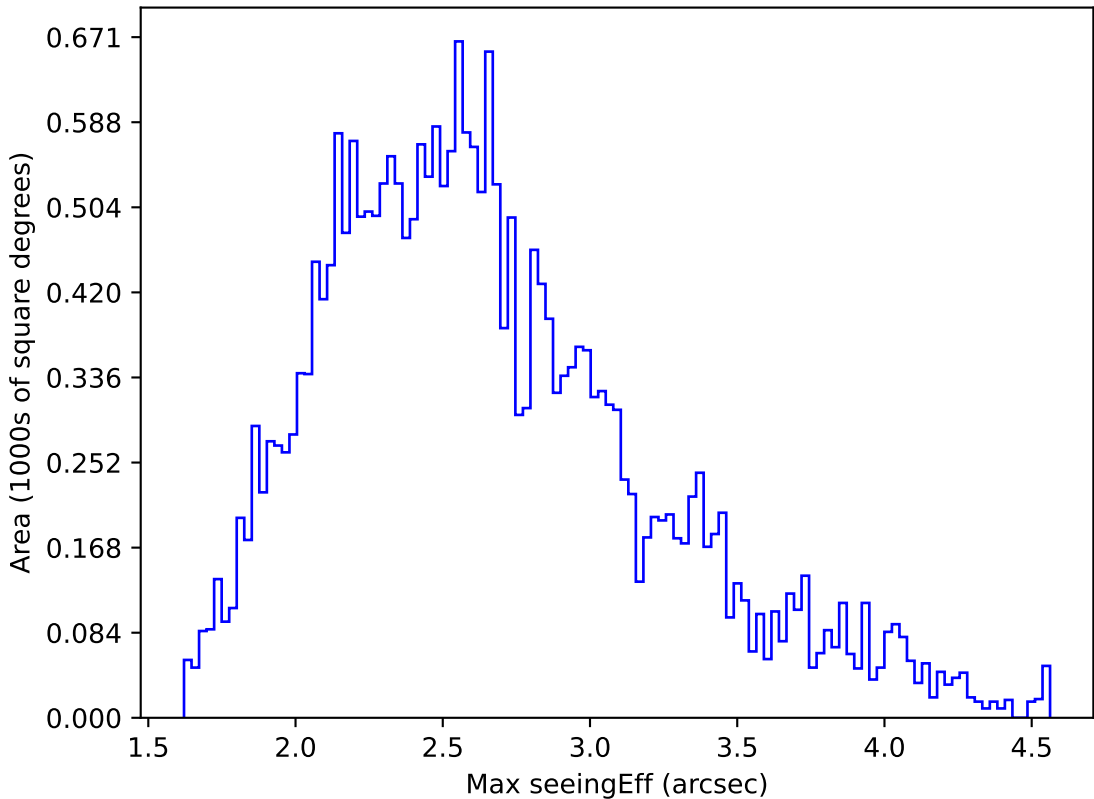
ddf_loaded_half_fl1_v3.4_10yrs All sky r band: Max seeingEff
