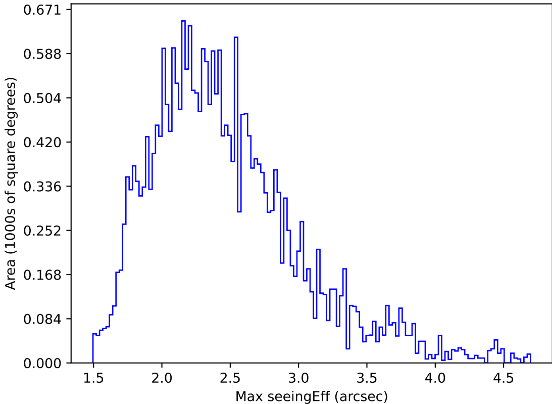
ddf_loaded_half_fl1_v3.4_10yrs All sky g band: Max seeingEff
