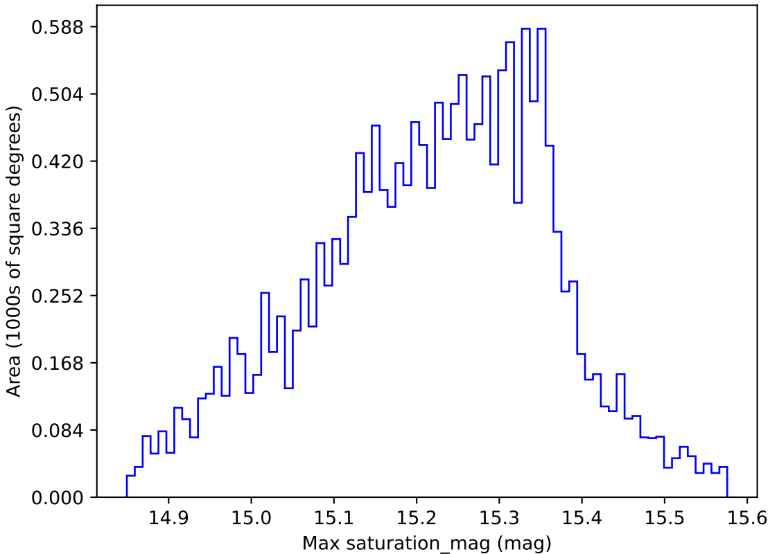
ddf_loaded_half_fl1_v3.4_10yrs WFD z band: Max saturation_mag
