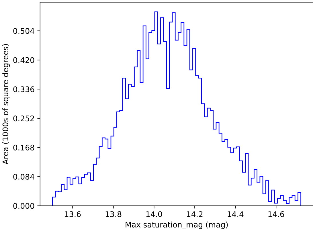
ddf_loaded_half_fl1_v3.4_10yrs WFD u band: Max saturation_mag
