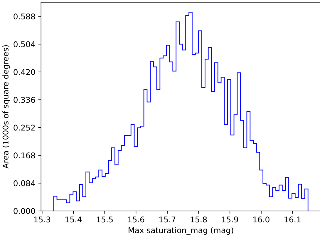
ddf_loaded_half_fl1_v3.4_10yrs WFD r band: Max saturation_mag
