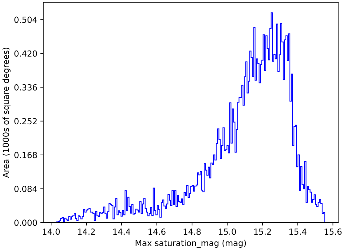
ddf_loaded_half_fl1_v3.4_10yrs All sky z band: Max saturation_mag
