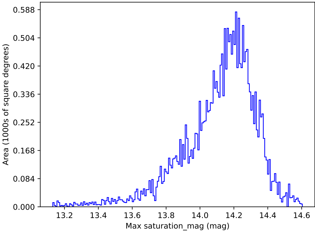
ddf_loaded_half_fl1_v3.4_10yrs All sky y band: Max saturation_mag
