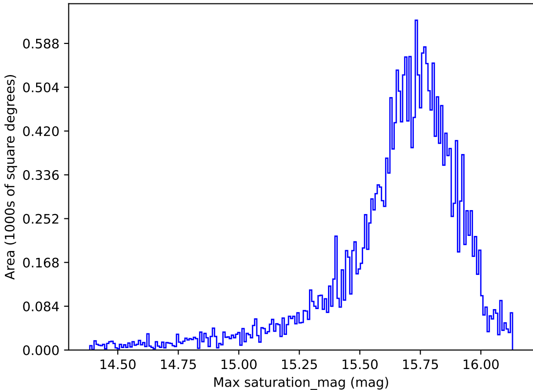
ddf_loaded_half_fl1_v3.4_10yrs All sky r band: Max saturation_mag
