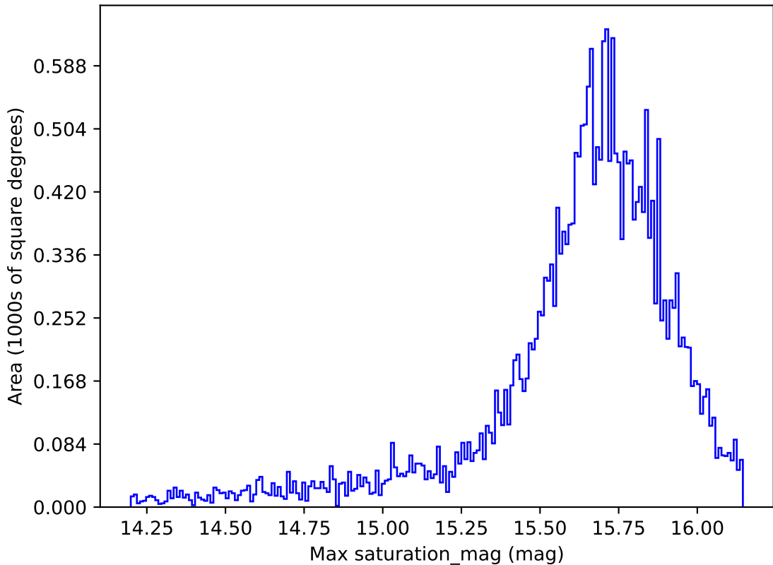
ddf_loaded_half_fl1_v3.4_10yrs All sky g band: Max saturation_mag
