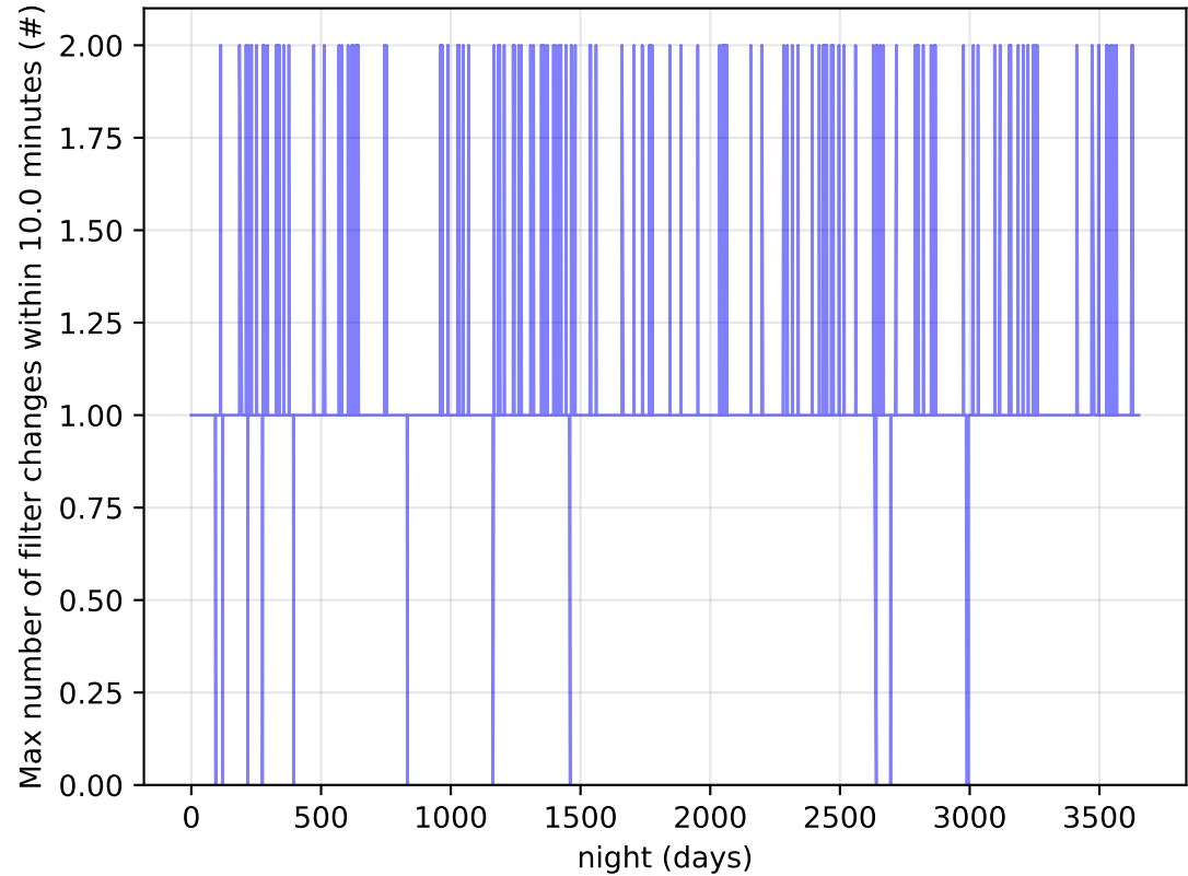
ddf_loaded_half_fl1_v3.4_10yrs Per Night: Max number of filter changes within 10.0 minutes
