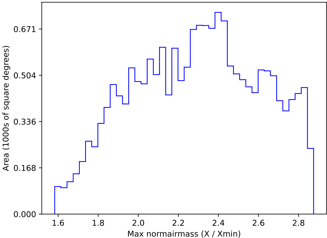
ddf_loaded_half_fl1_v3.4_10yrs WFD z band: Max normairmass
