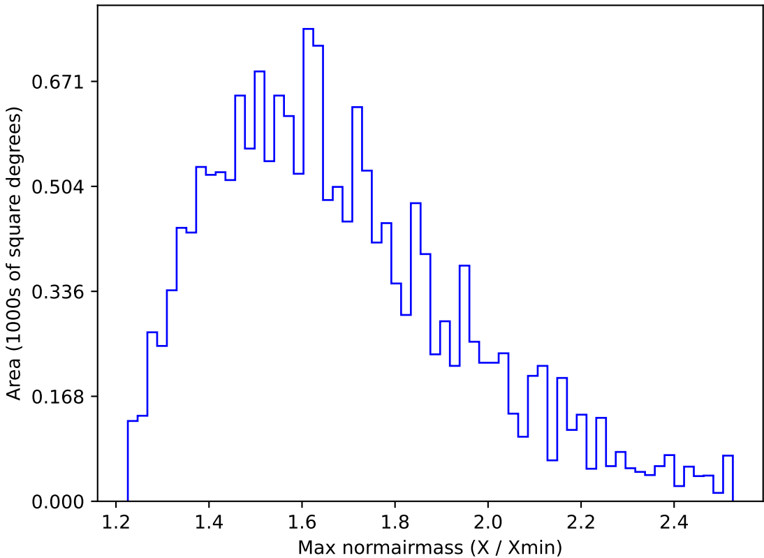
ddf_loaded_half_fl1_v3.4_10yrs WFD u band: Max normairmass
