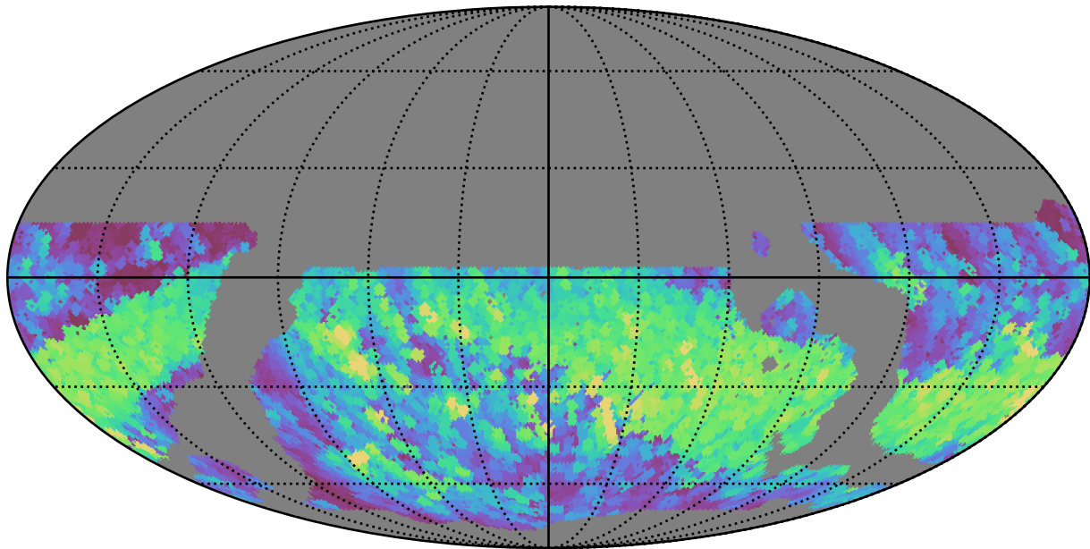
ddf_loaded_half_fl1_v3.4_10yrs WFD r band: Max normairmass
